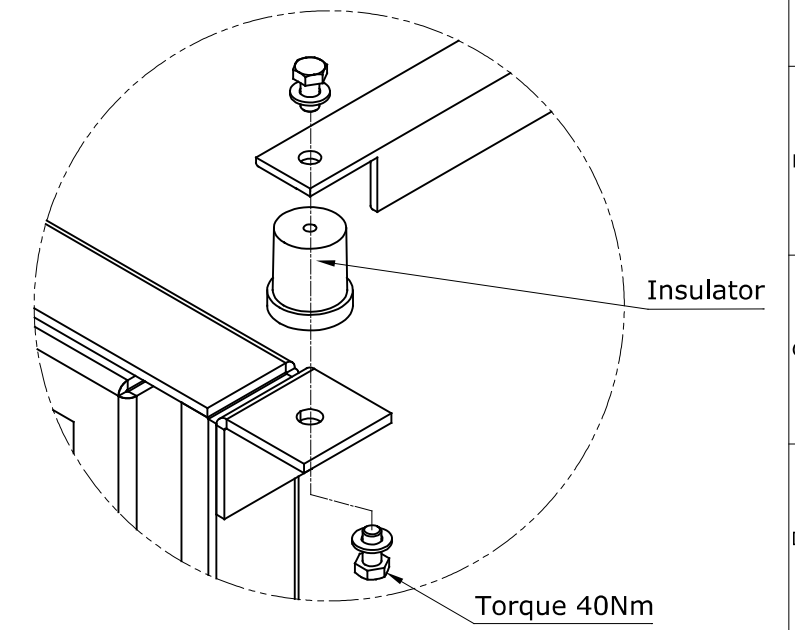
View - A Details Anchor Bolt assembly Enlarged View
