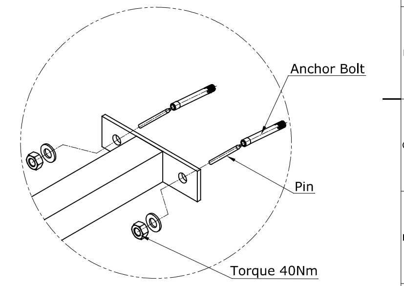
View - B Details Angle Bracket assembly Enlarged View
